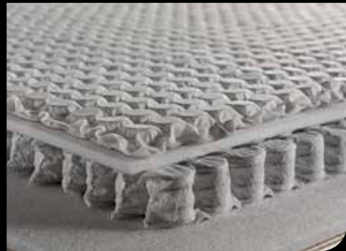
molle/springs ELASYSTEM Micro Pocket Springs h2
